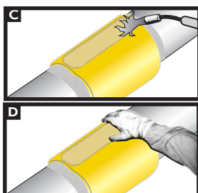
14A Gently heat the closure and pat it down with a gloved hand. Repeating this procedure, move from one side to the other. Smooth any wrinkles by gently working them outward from the centre of the closure with a roller.
