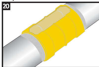
20 Visually inspect the installed sleeve for the following: • Sleeve is in full contact with the steel joint. • Adhesive flows beyond both sleeve edges. • No cracks or holes in sleeve backing.
