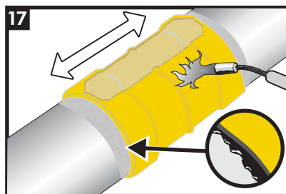
17 Shrinking has been completed when the adhesive begins to ooze at the sleeve edges all around the circumference. Finish shrinking the sleeve with long horizontal strokes over the entire surface to ensure a uniform bond.
