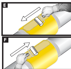
14A Gently heat the closure and pat it down with a gloved hand. Repeating this procedure, move from one side to the other. Smooth any wrinkles by gently working them outward from the centre of the closure with a roller.
