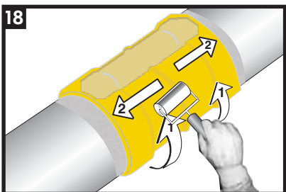
18 While the sleeve is still hot and soft, use a hand roller to gently roll the sleeve surface and push any trapped air up and out of the sleeve, as shown above. If necessary, reheat to roll out air.
